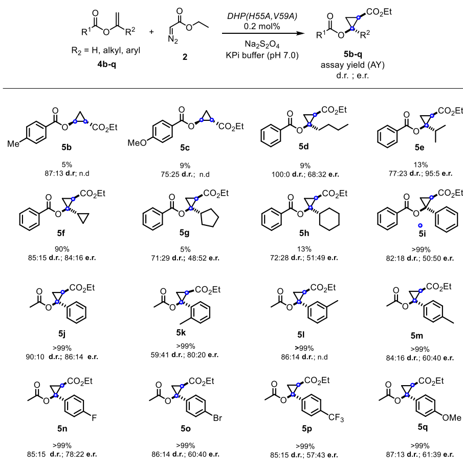
Figure 3. Substrate scope for DHP(H55A, V59A)-catalyzed cyclopropanation of vinyl esters. Reaction conditions: 20 \mu M enzyme, 2.5 mM substrate, 10 mM EDA, 10 mM dithionite, 10% MeOH, KPi buffer (50 mM, pH 7), anaerobic, 4 h. Assay yield, diastereomeric ratio (dr), and enantiomeric ratio (er) were determined by chiral GC-FID and SFC analysis using calibration curves with authentic (racemic) standards. For compounds 5d–5q , only relative configuration was assigned. See the Experimental Section for further details on stereochemical assignments.
